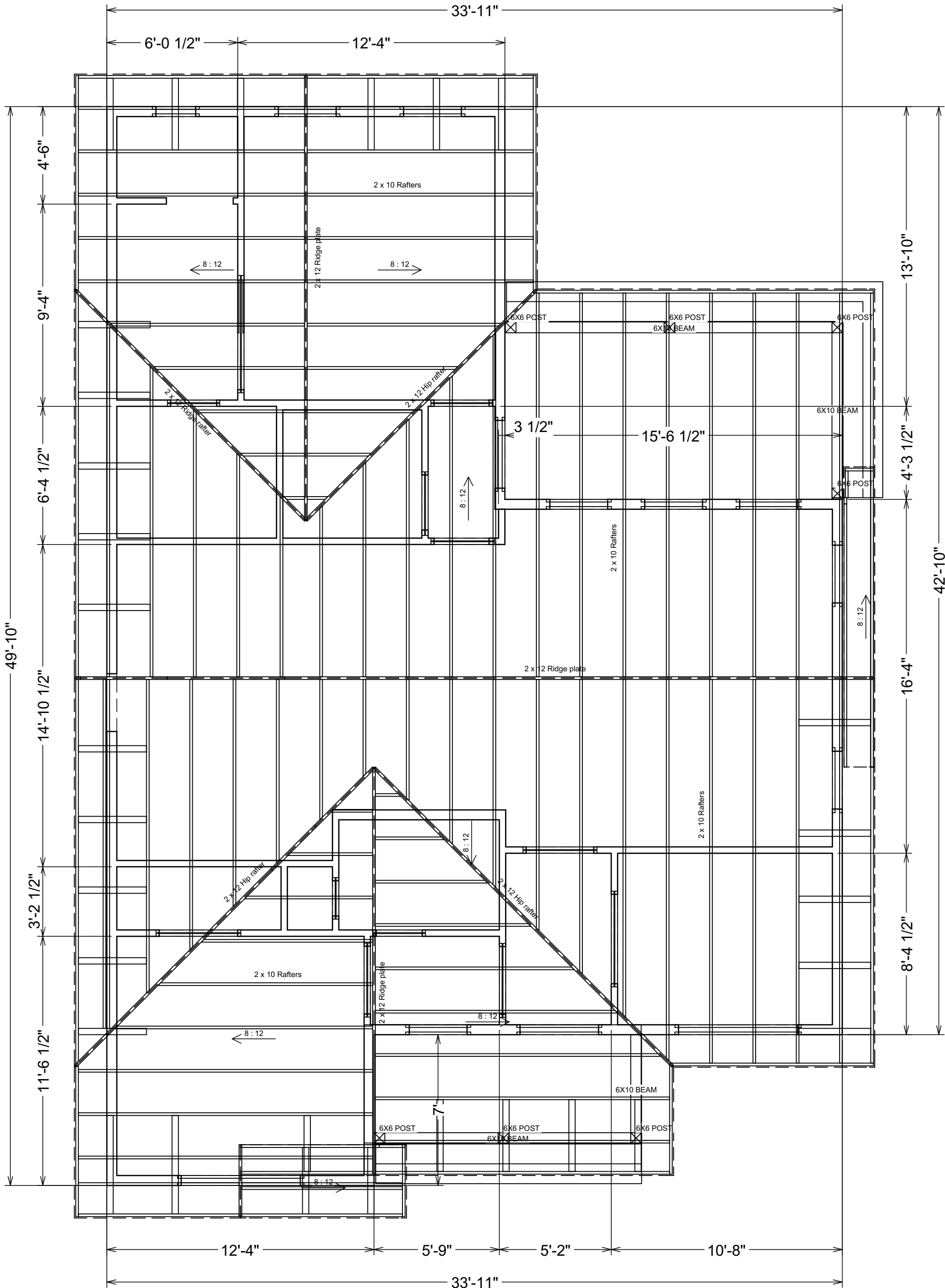
1 Framing, Roof Plan View.
