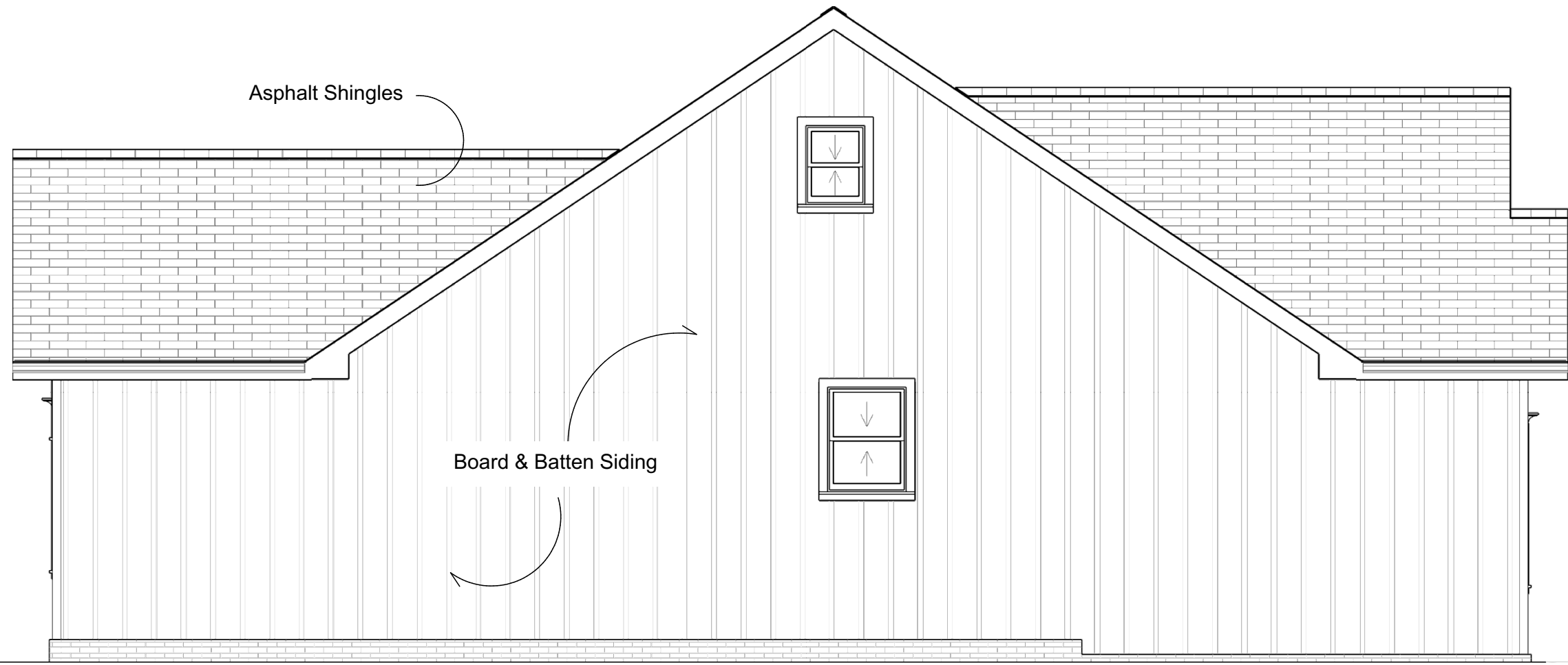
AR 04 SCALE 1/2"=1'-0"
