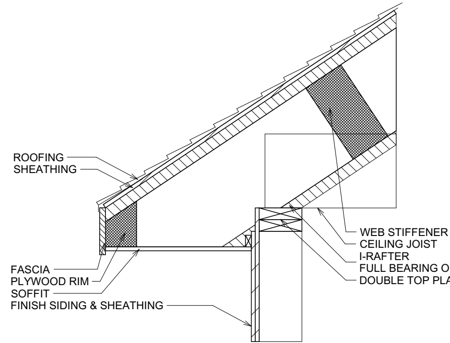
2 Soffited Eave Details.
